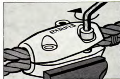
Working diagram of wirelock in wire rope loop
